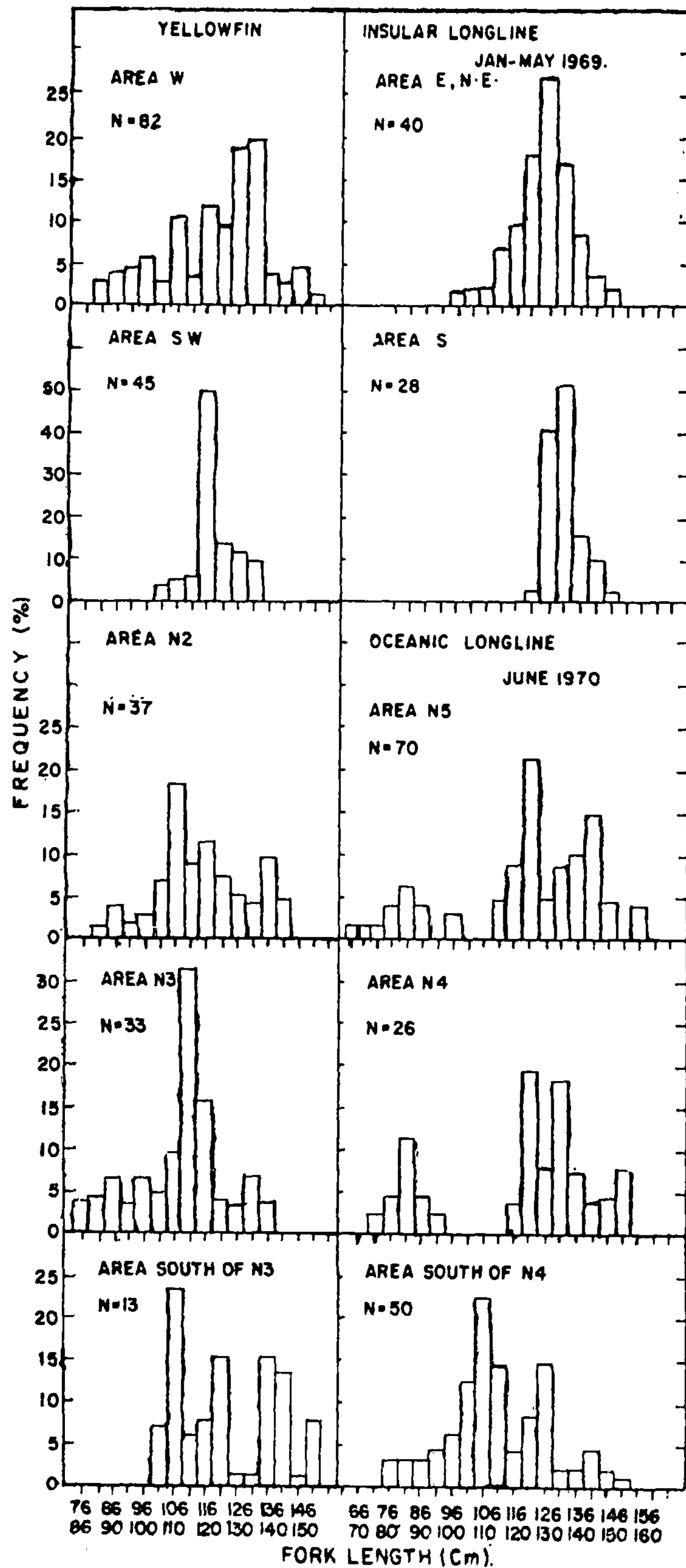
Fig. 7. Length frequency distributions for yellowfin tuna caught by longline in the different oceanic areas and insular range
