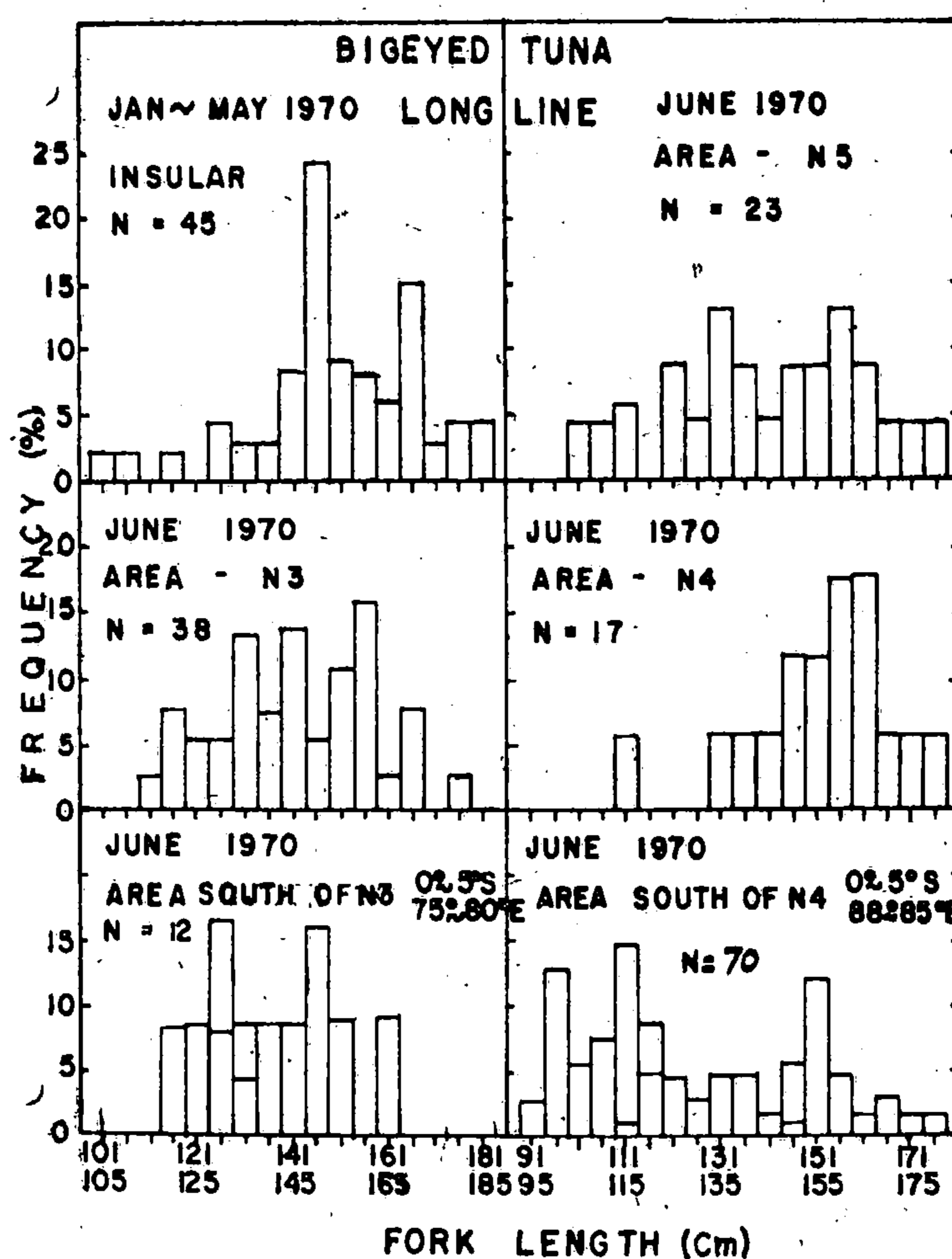
Fig. 8. Length frequency distributions for Bigeye tuna caught by longline in the insular and oceanic areas
