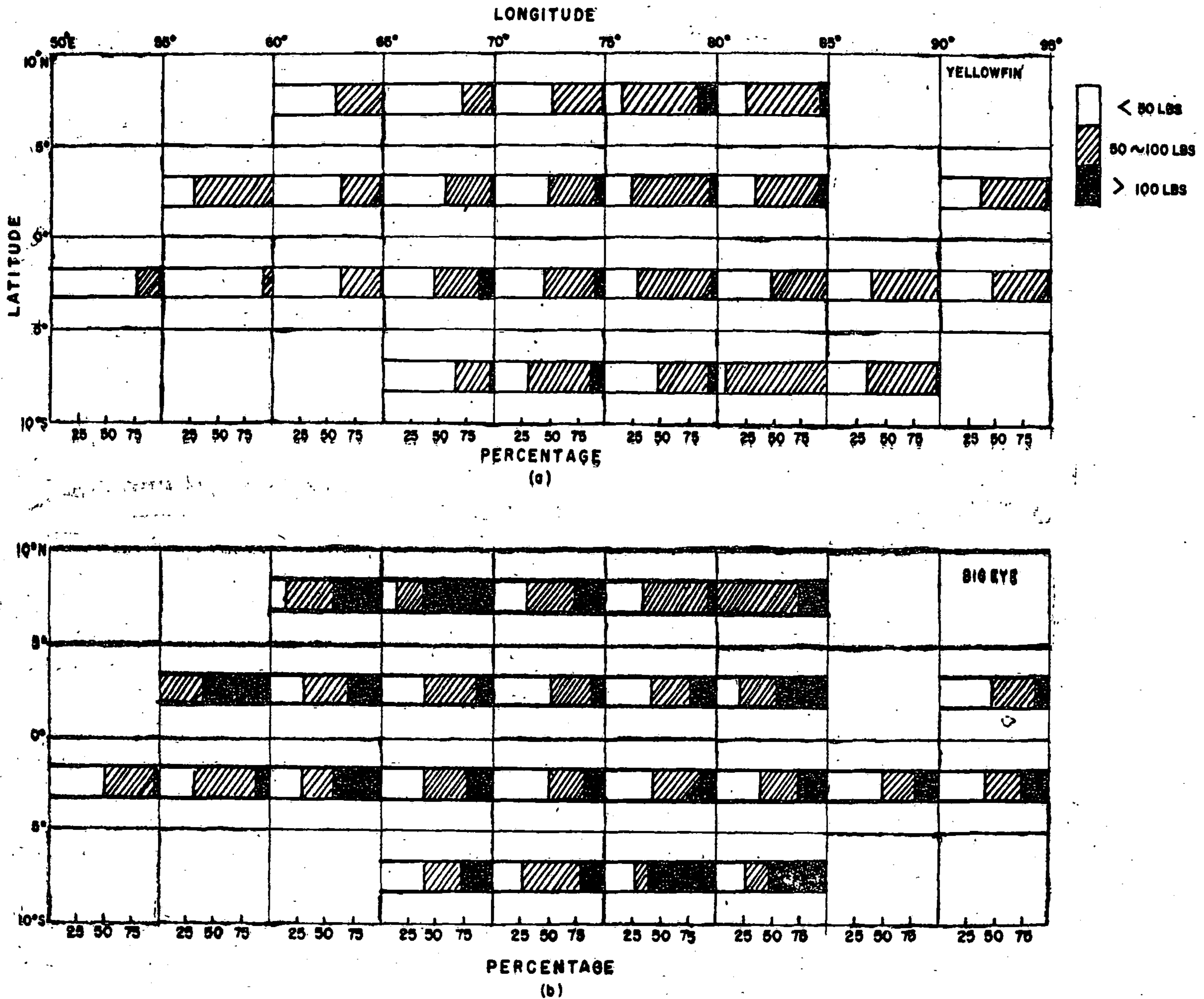
Fig. 9. Percentage composition by weight of Yellowfin and Bigeye tunas caught in different areas of the Indian Ocean.
