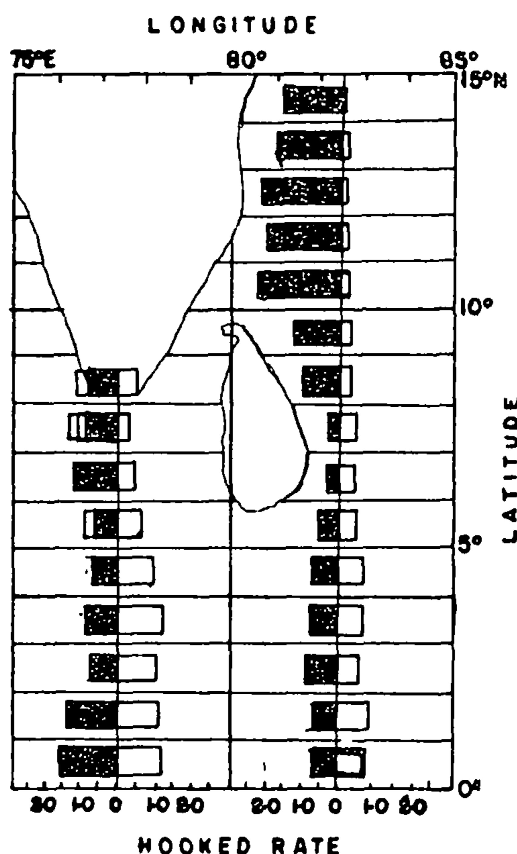
Fig. 3. Hooked rates (%) of yellowfin (shaded) and Bigeye tunas in the oceanic range
