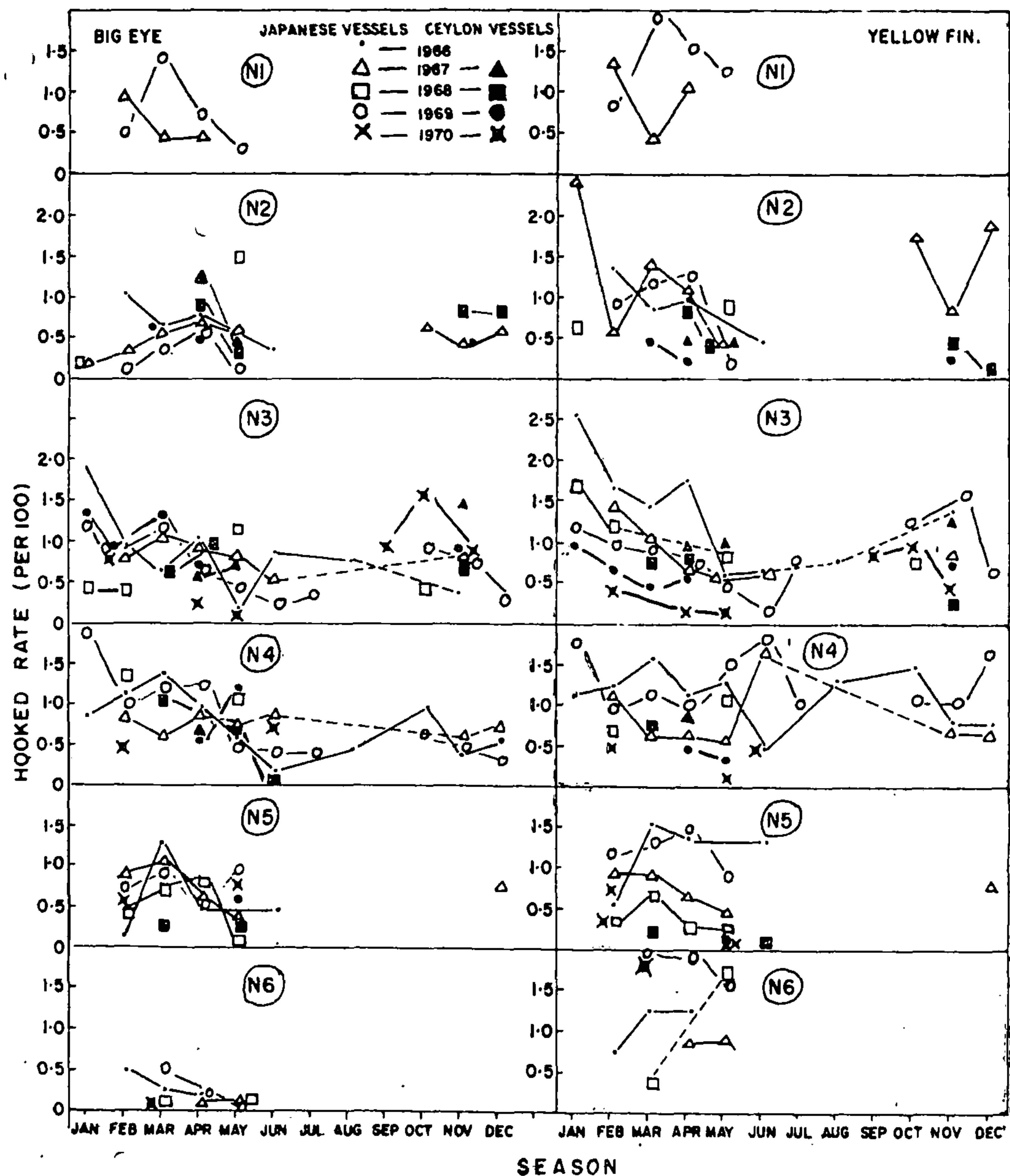
Fig. 5. Seasonal variation in the hooked rates of Bigeye and yellowfin tunas in the areas of the oceanic range
