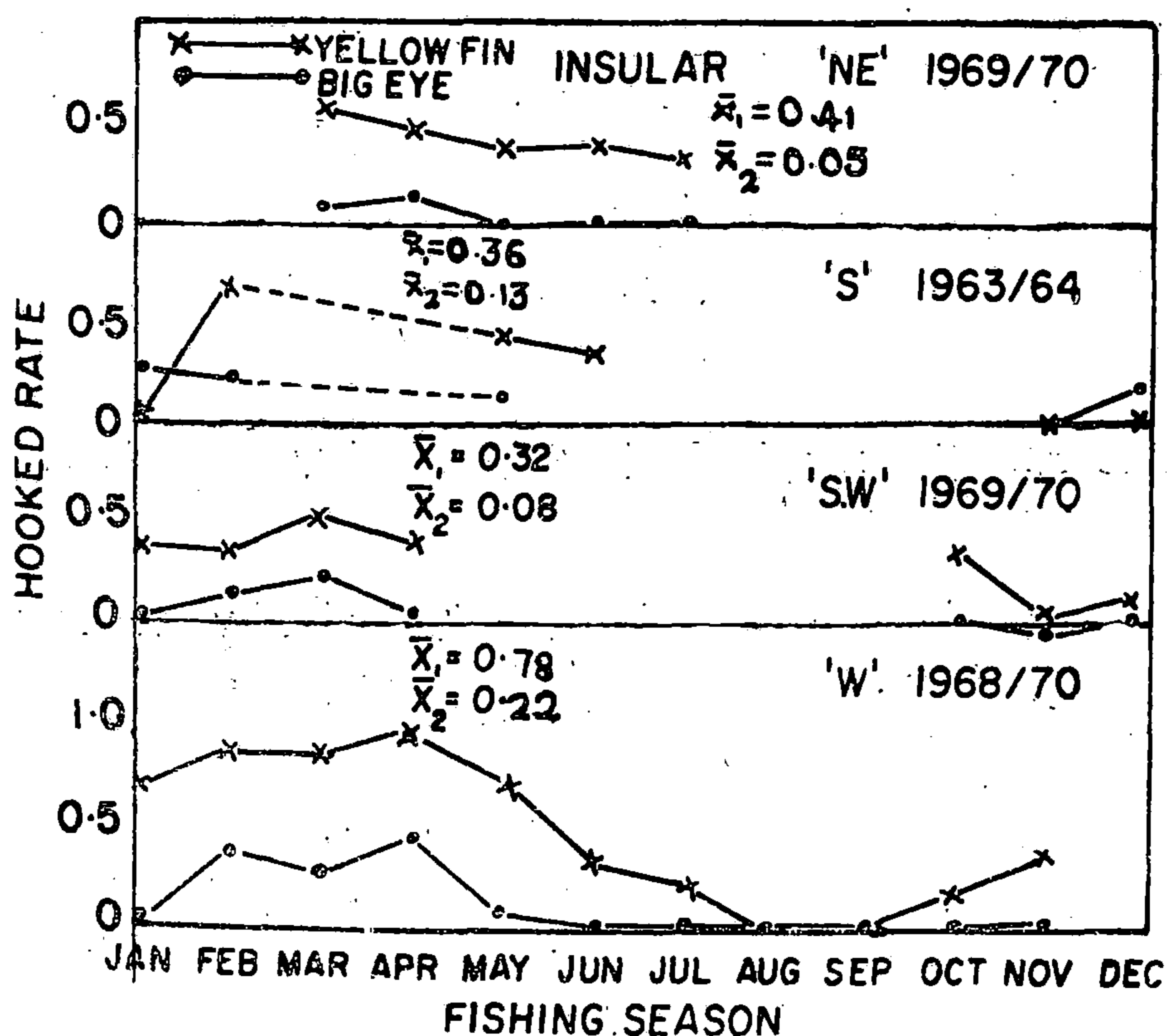
Fig. 4. Seasonal variations in the hooked rates of yellowfin and Bigeye tunas in the inshore areas
