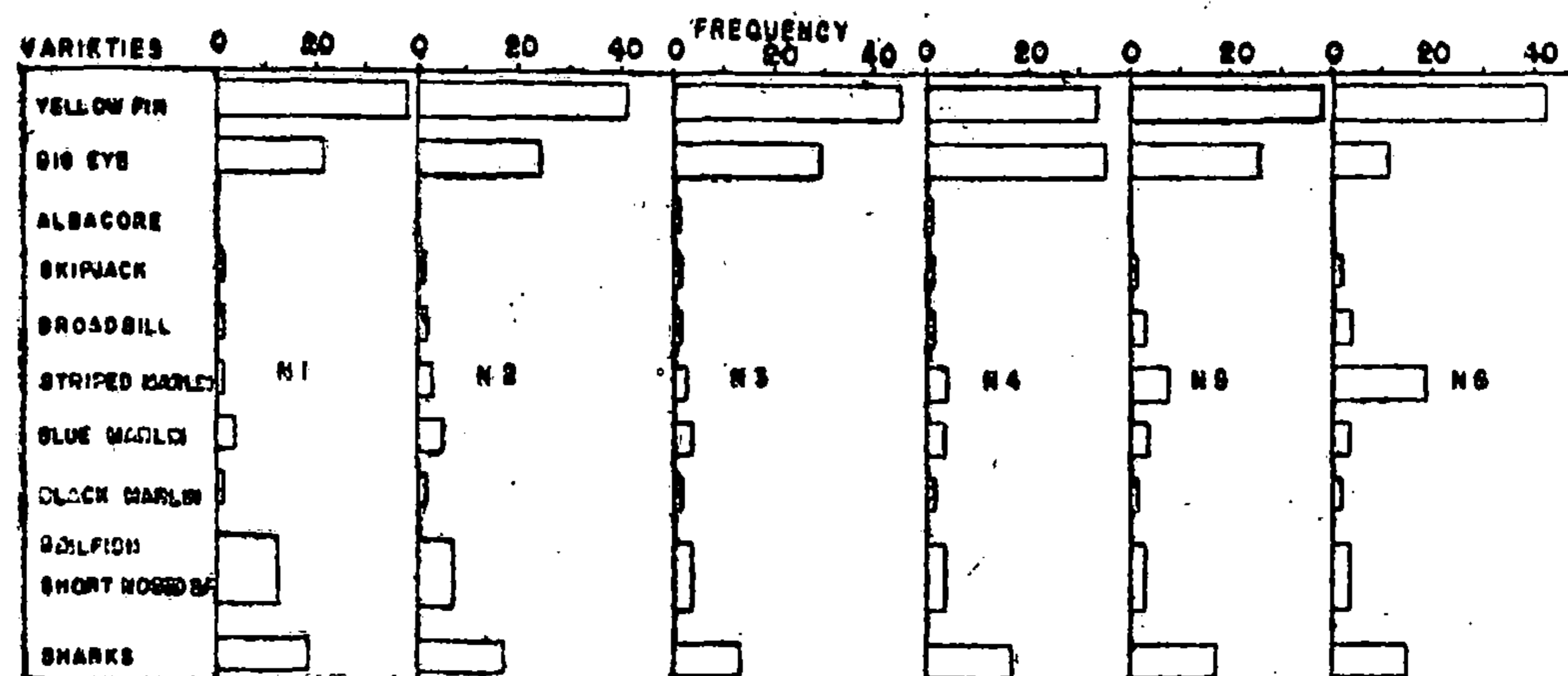
Fig. 2. The percentage species Composition in the longline catches, in the areas of the Oceanic range
