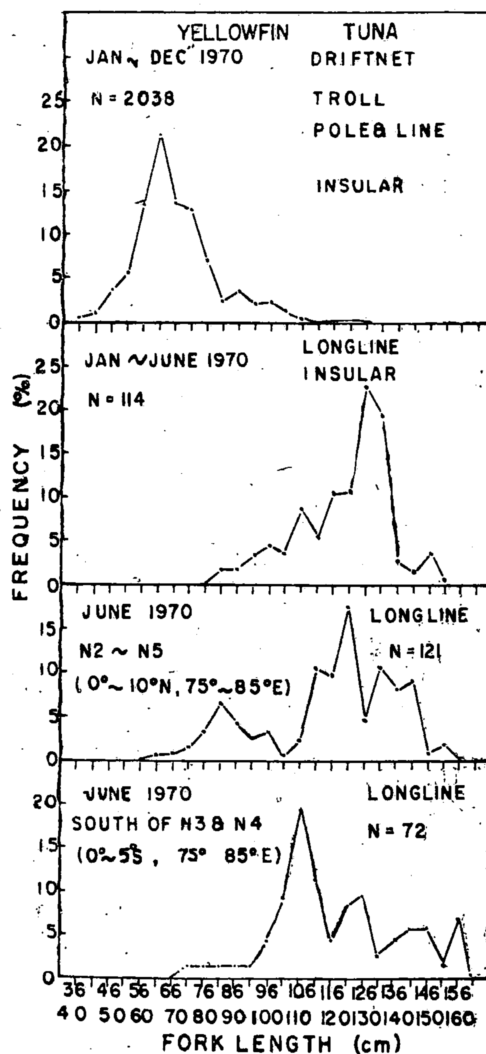
Fig. 6. Length frequency distributions of yellowfin tuna in the surface and deepswimming layers of the insular and oceanic ranges
