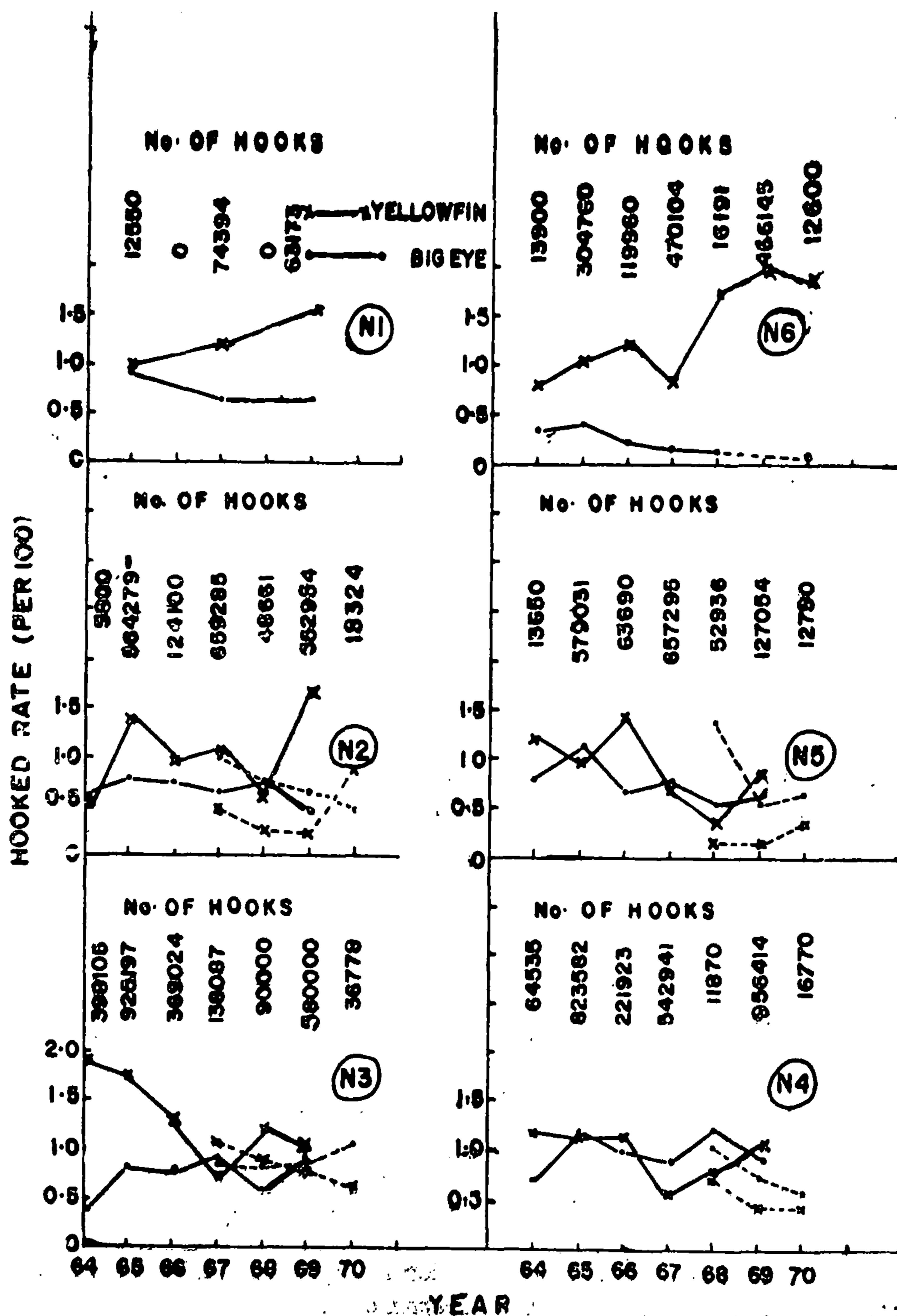
Fig. 10. Annual variations in the effort and hooked rates for Yellowfin and Bigeye tunas in the oceanic areas. (Complete line for Japan and incomplete lines for Ceylon).
